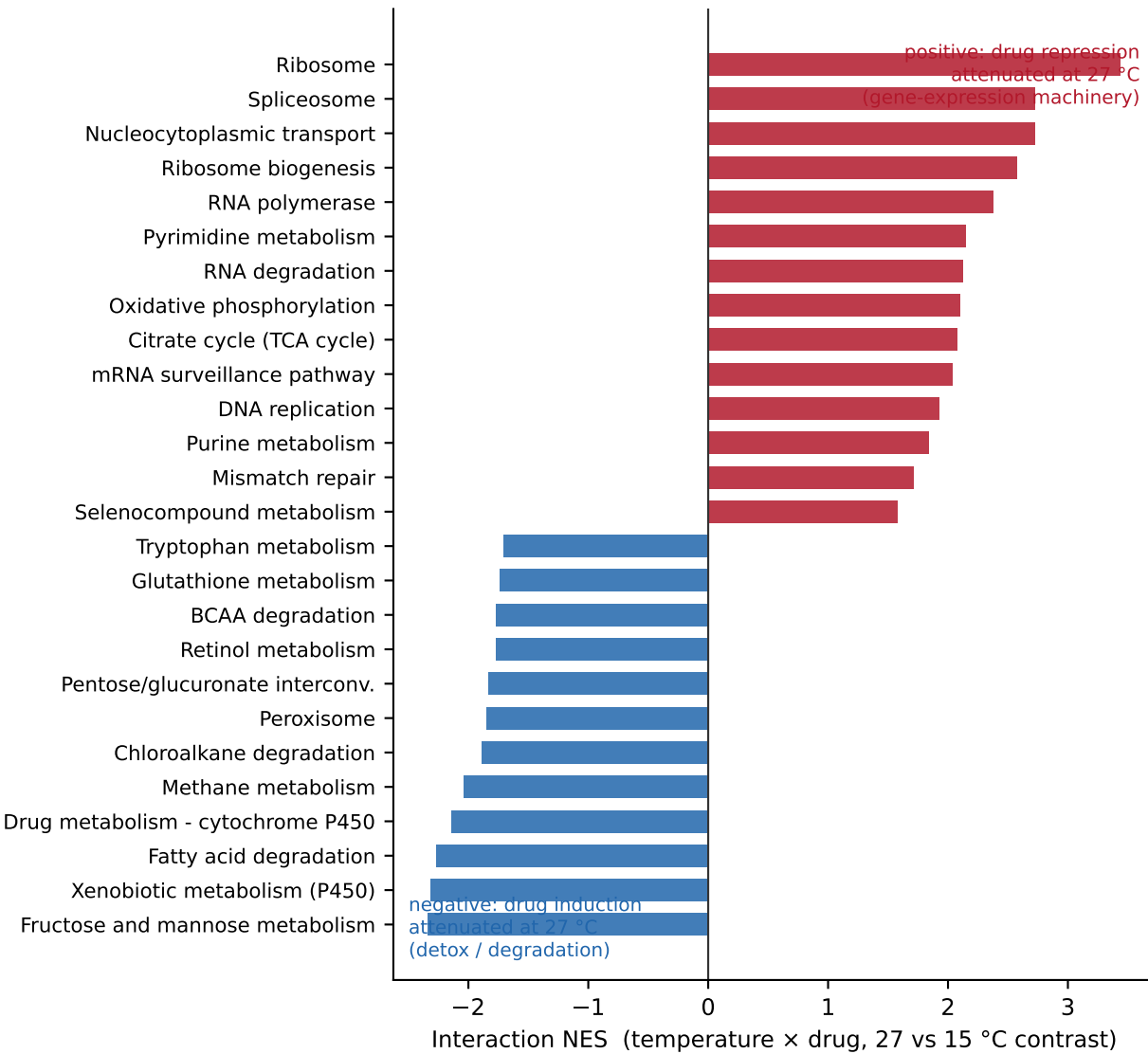
Pathway-level temperature × drug interaction (GSEA, FDR < 0.05; n = 26 of 105 pathways)
