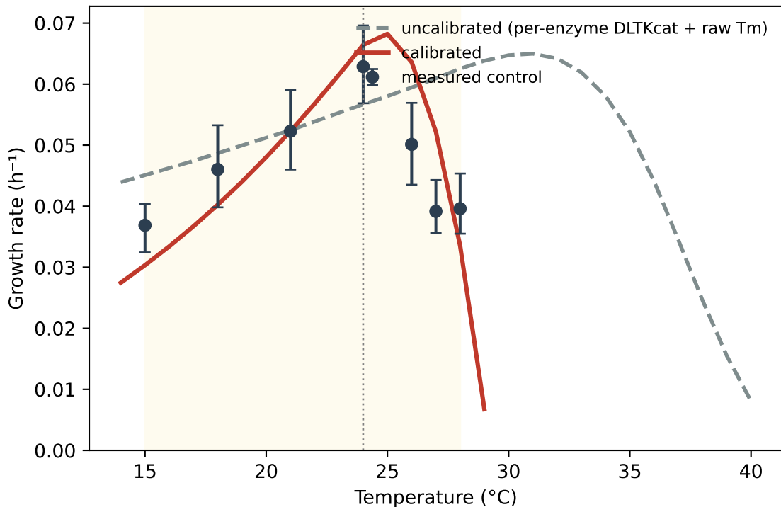
Proper uncalibrated ETC-GEM TPC (per-enzyme sequence kinetics)
