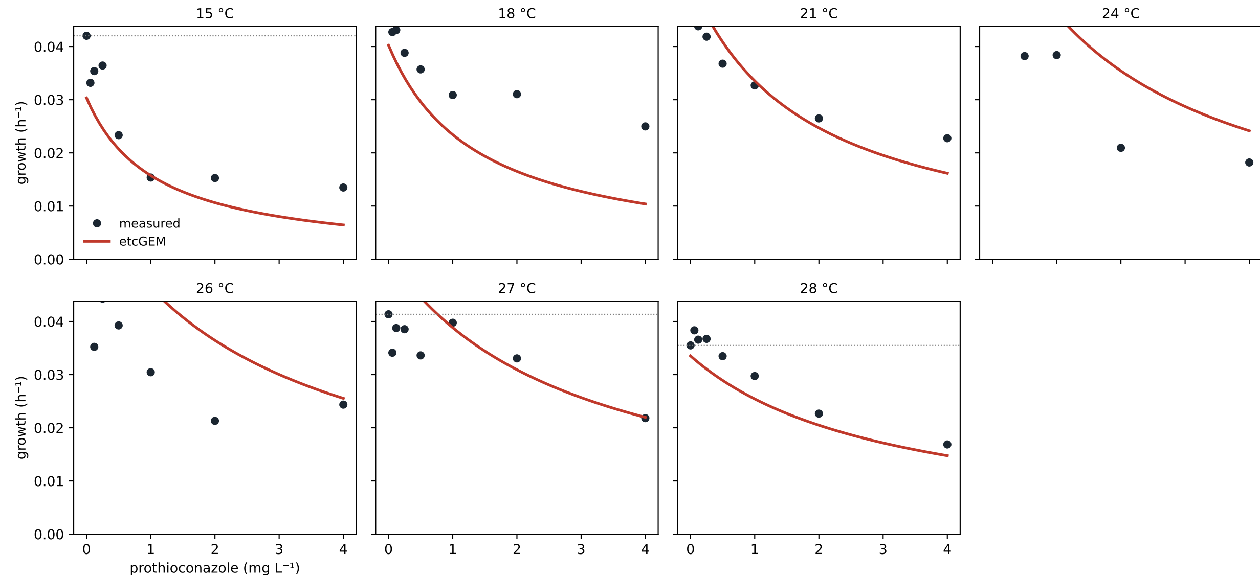
Calibrated etcGEM growth surface: control (mechanistic) + graded drug (fitted) [abs r=0.82, interaction r=0.84]
