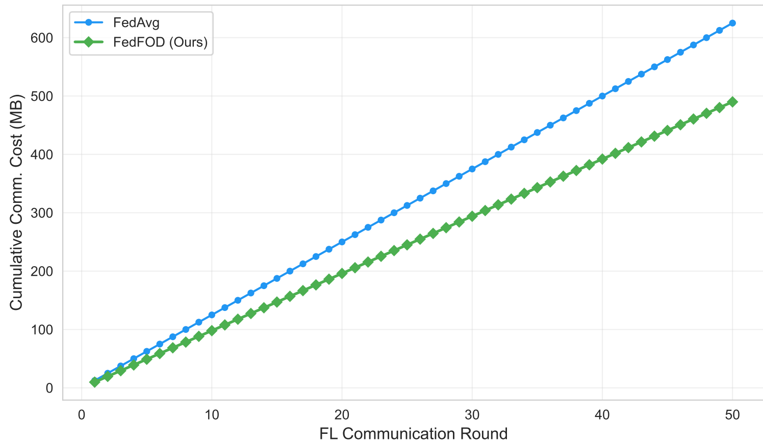
Cumulative Communication Cost
