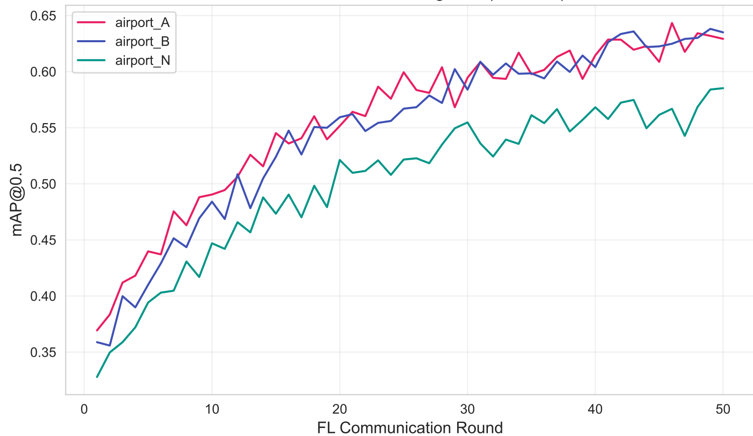
Per-Client mAP Convergence (FedFOD)
