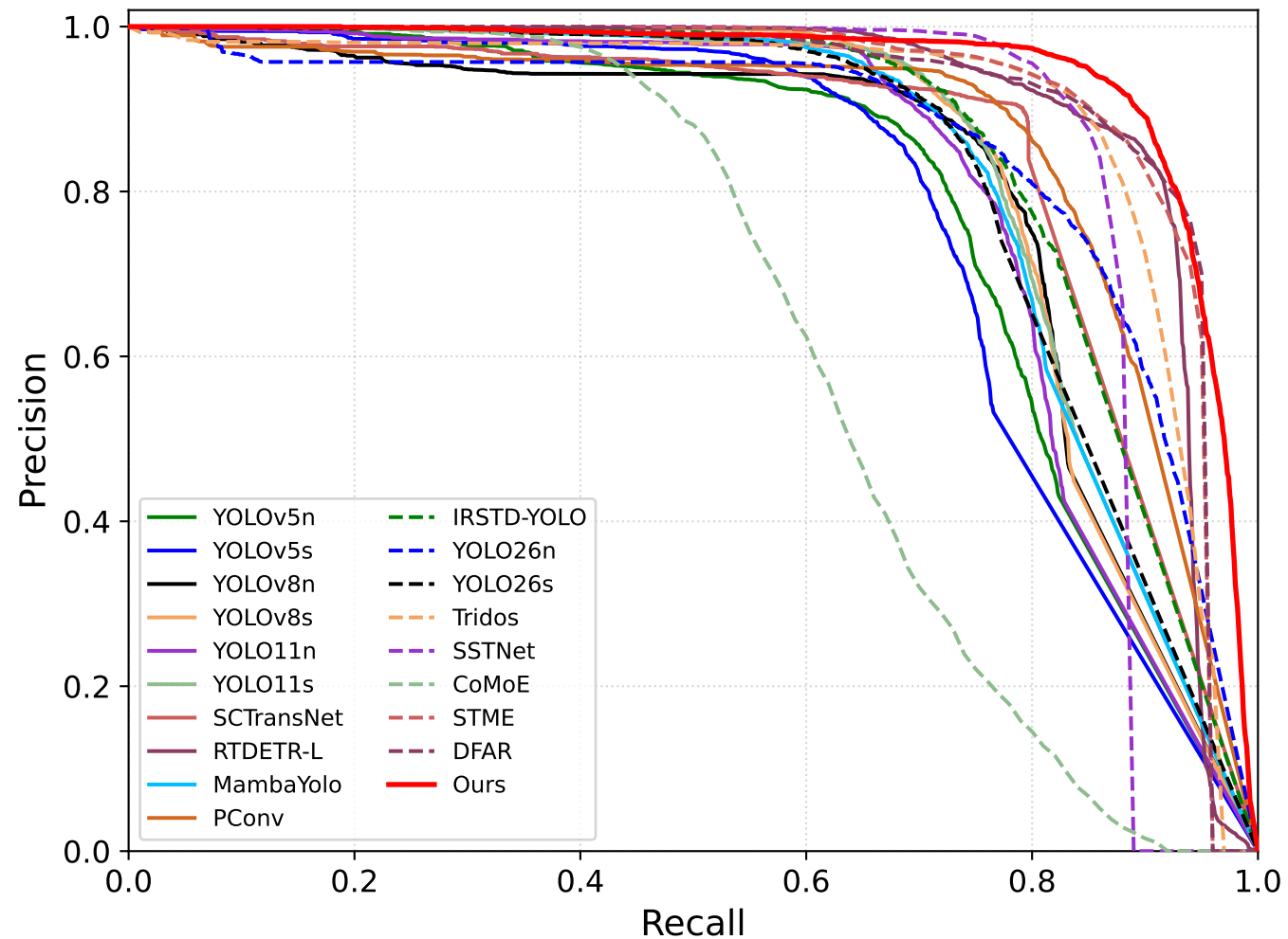
PR Curve on DAUB
