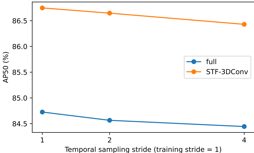
DAUB: 4,683 common keyframes; fixed seed 0
