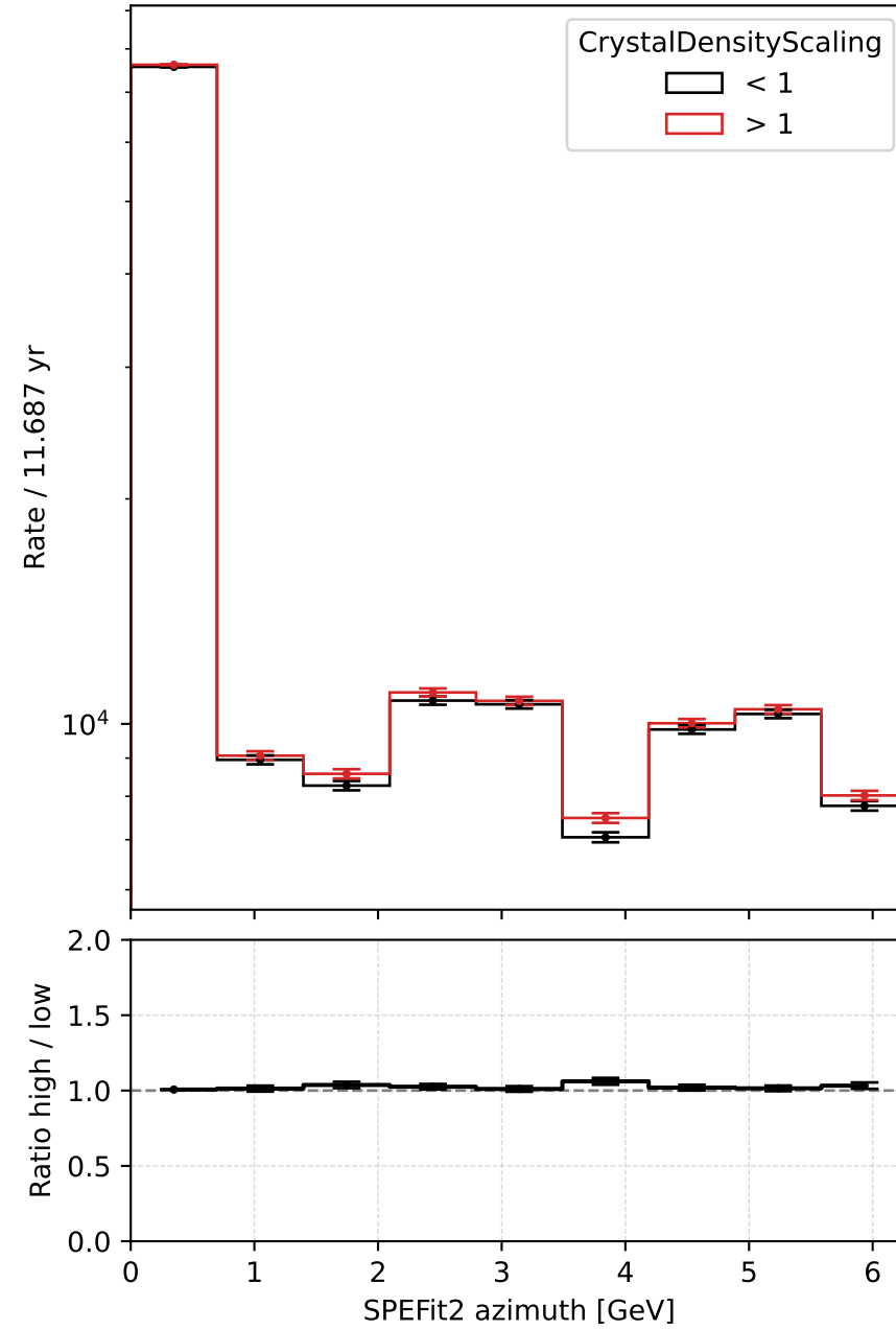
NuMu astro, \gamma = 2.87 , \phi_0 = 2.12 , HESE
