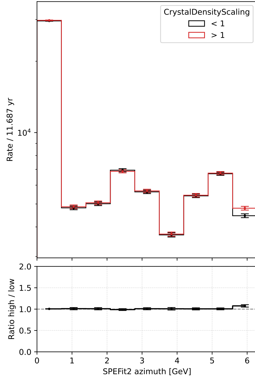
NuE astro, \gamma = 2.87 , \phi_0 = 2.12 , HESE
