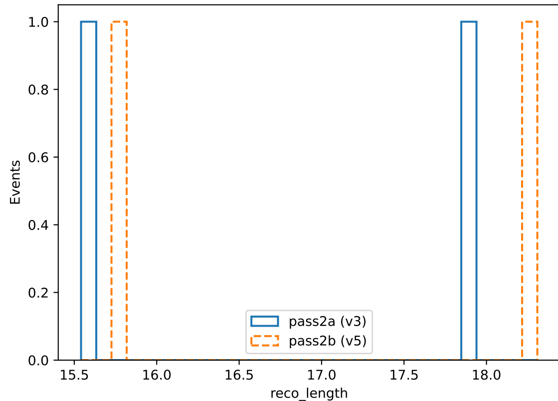
Distributions
