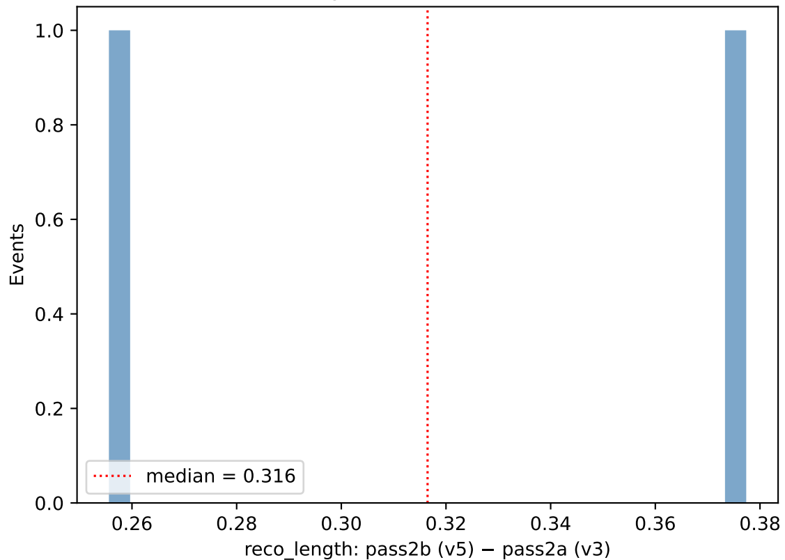
Event-by-event difference (N=2)
