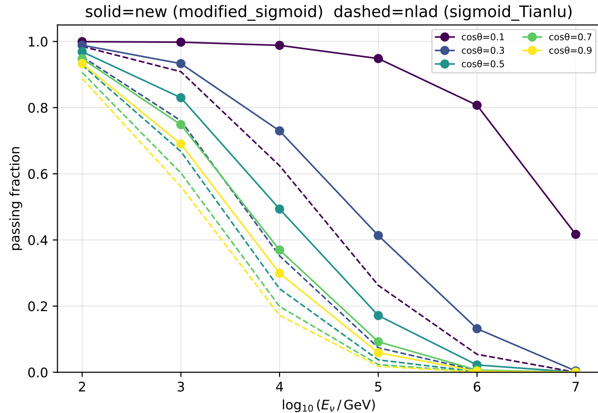
PF vs energy — conv nu_bar | depth=1950 m
