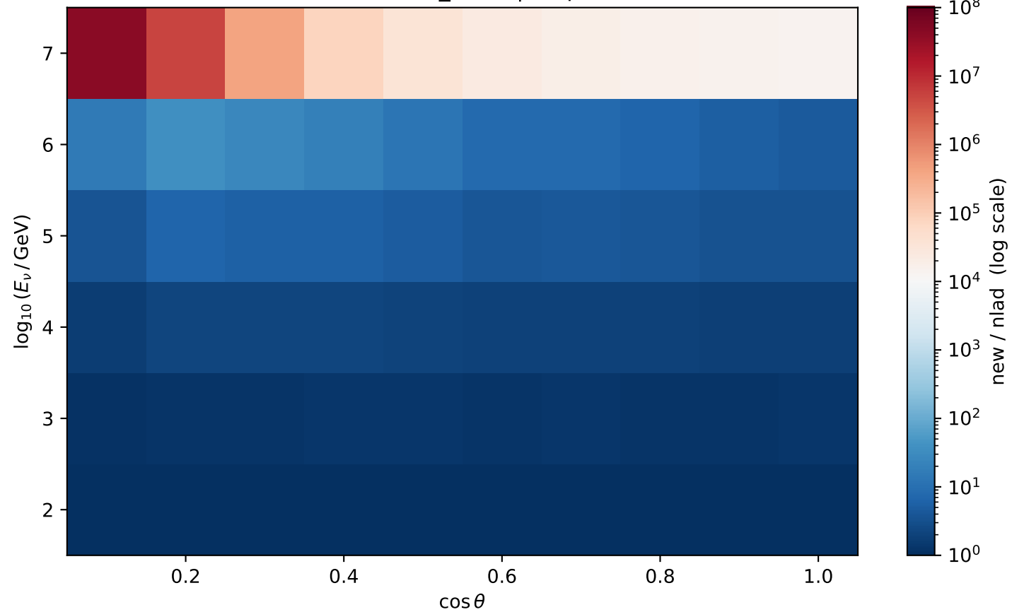
Ratio 2D — conv nu_ebar | depth=1950 m
