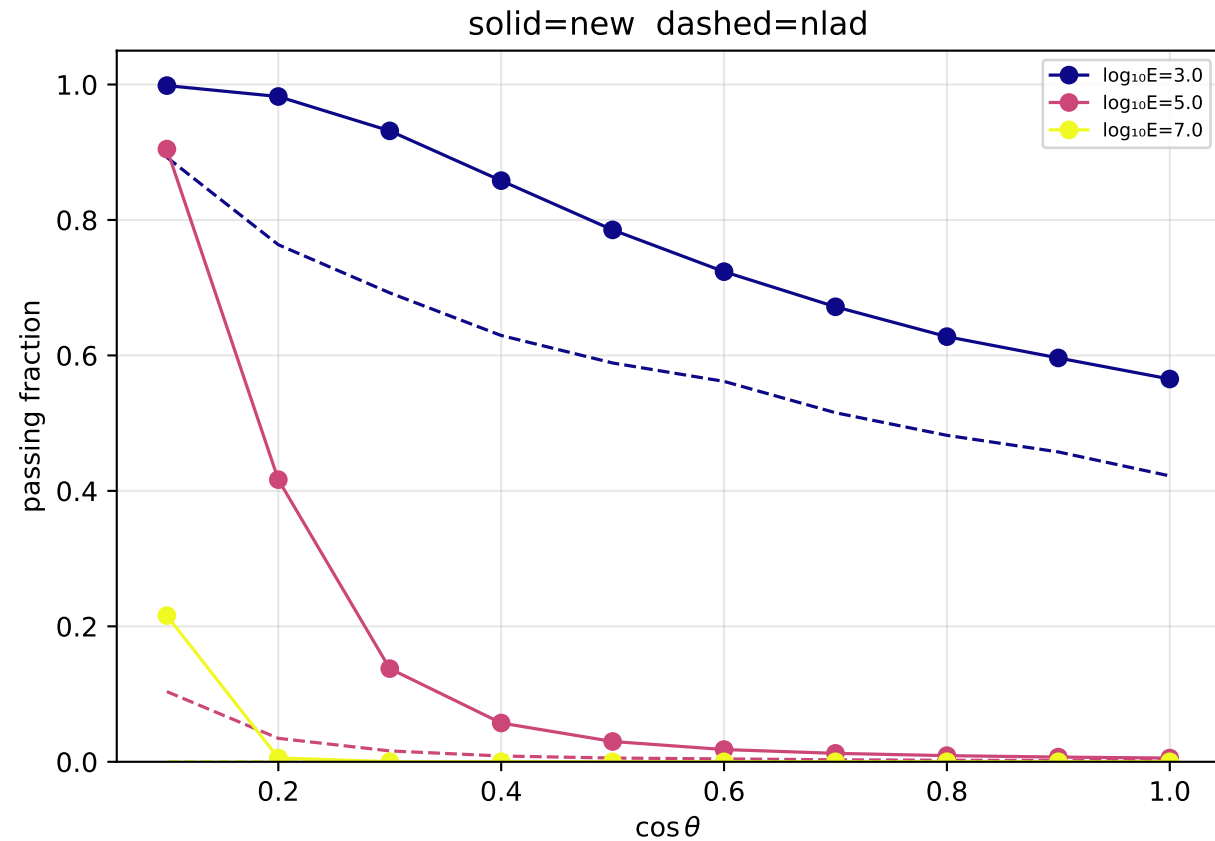
PF vs \cos \theta — conv nu_mu | depth=1950 m
