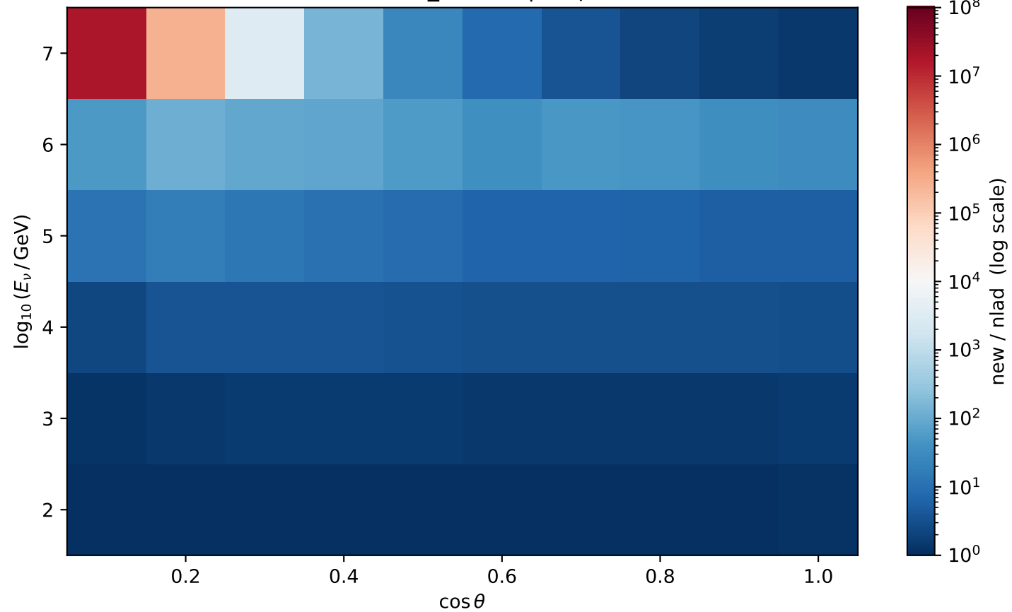
Ratio 2D — conv nu_mubar | depth=1950 m
