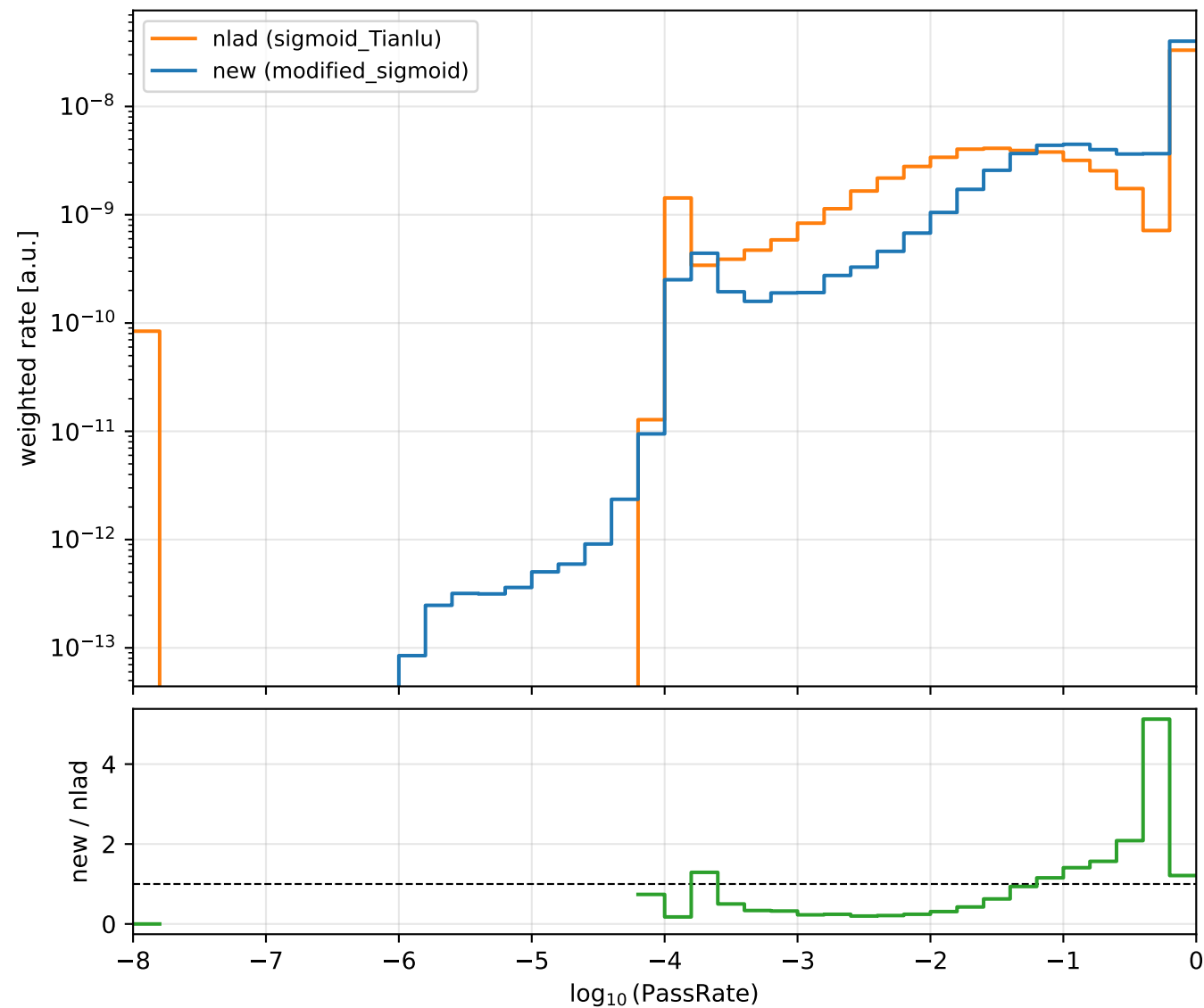
PassRate distribution | \bar{v}_e | PassRate_conv weight = fluxless_weight \times AstroFlux
