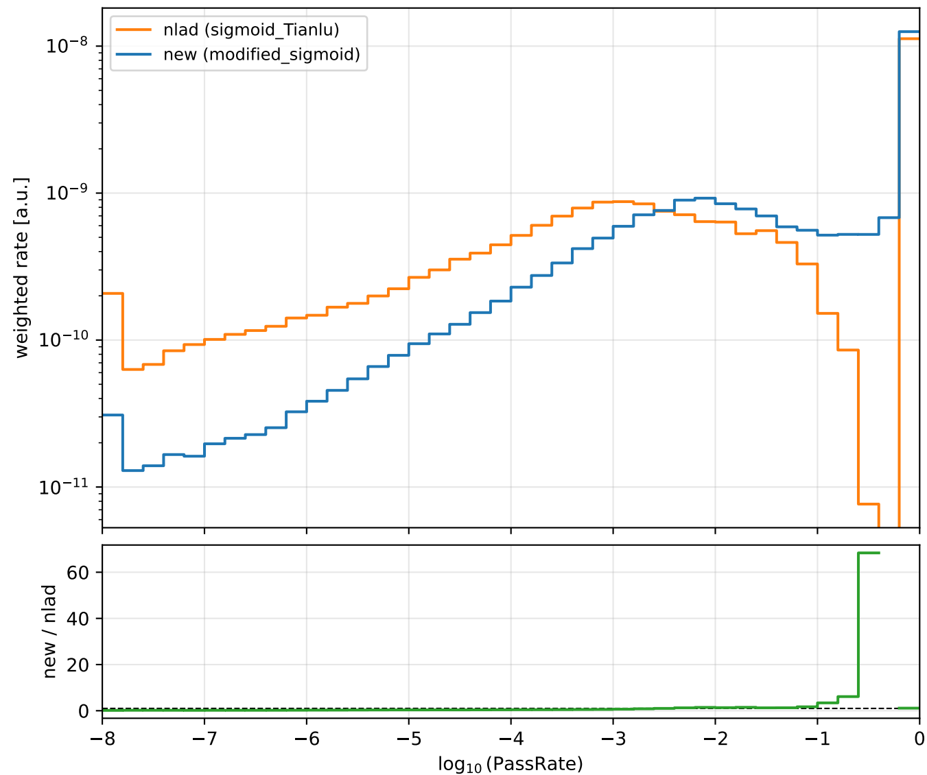
PassRate distribution | \bar{v}_\mu | PassRate_conv weight = fluxless_weight \times AstroFlux
