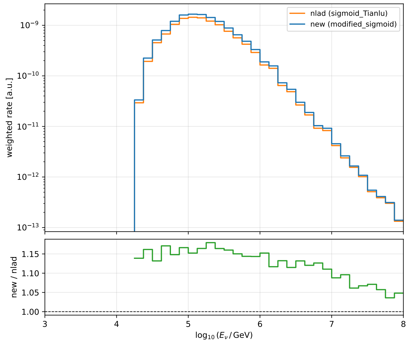
PassRate_conv | \bar{\nu}_\mu weight = fluxless_weight \times AstroFlux \times PassRate
