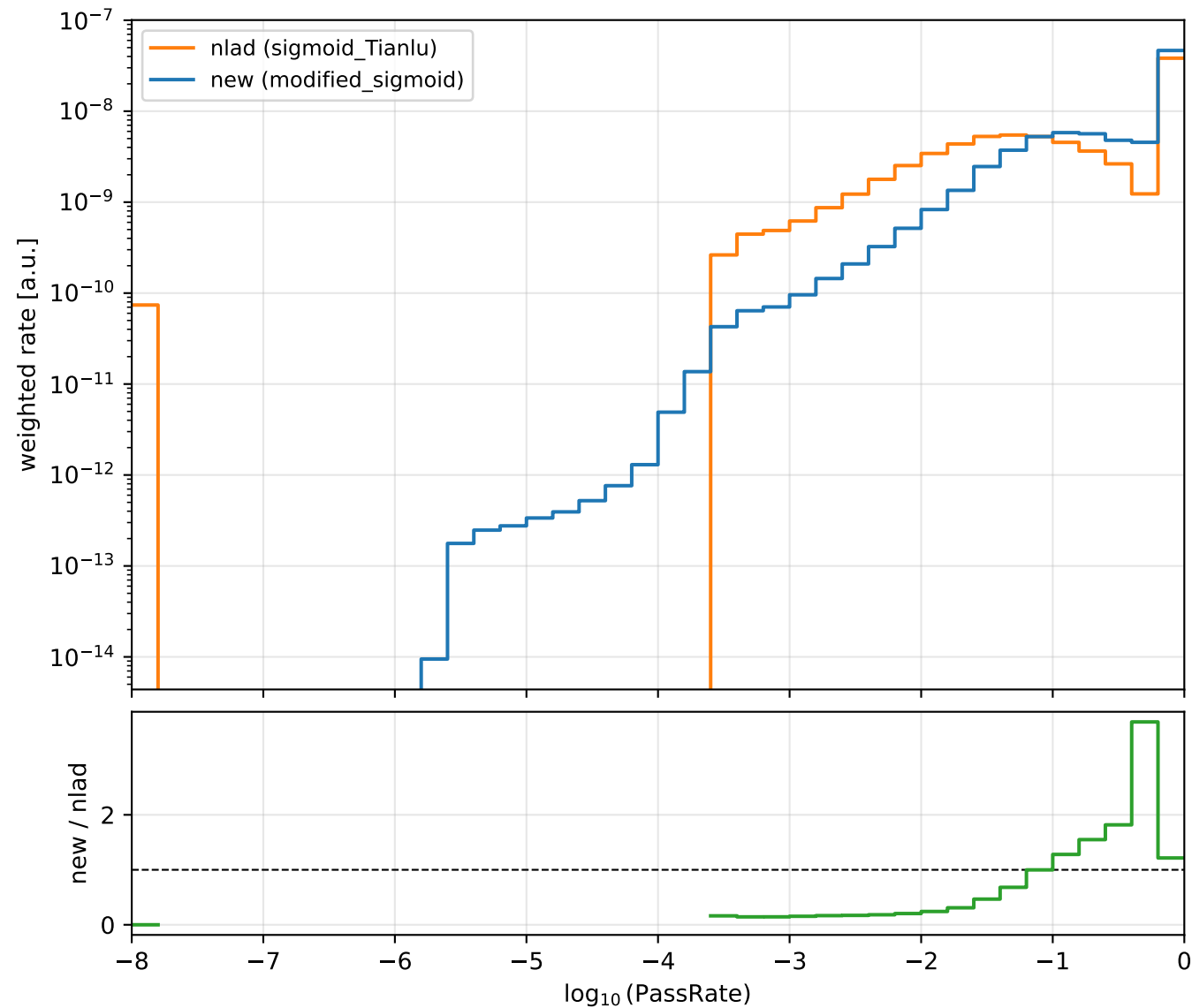
PassRate distribution | v_e | PassRate_conv weight = fluxless_weight \times AstroFlux
