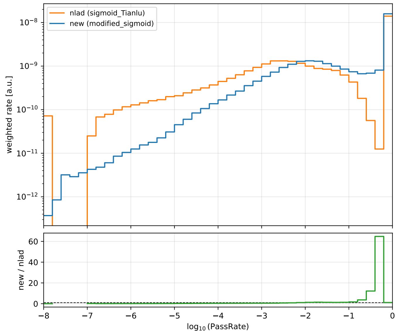
PassRate distribution | v_\mu | PassRate_conv weight = fluxless_weight \times AstroFlux
