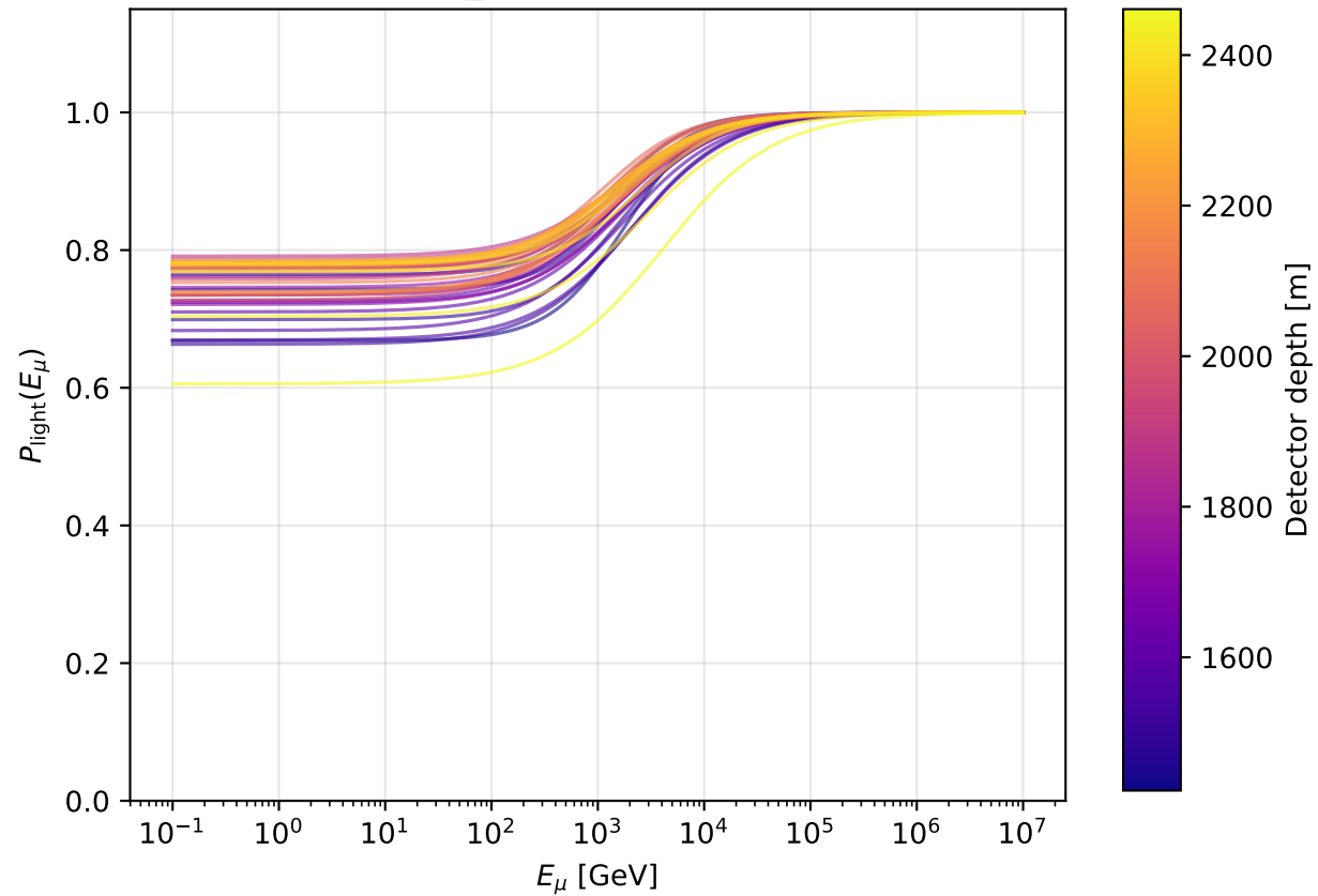
Old — sigmoid_Tianlu (39 slices, floor \approx 0.6 )
