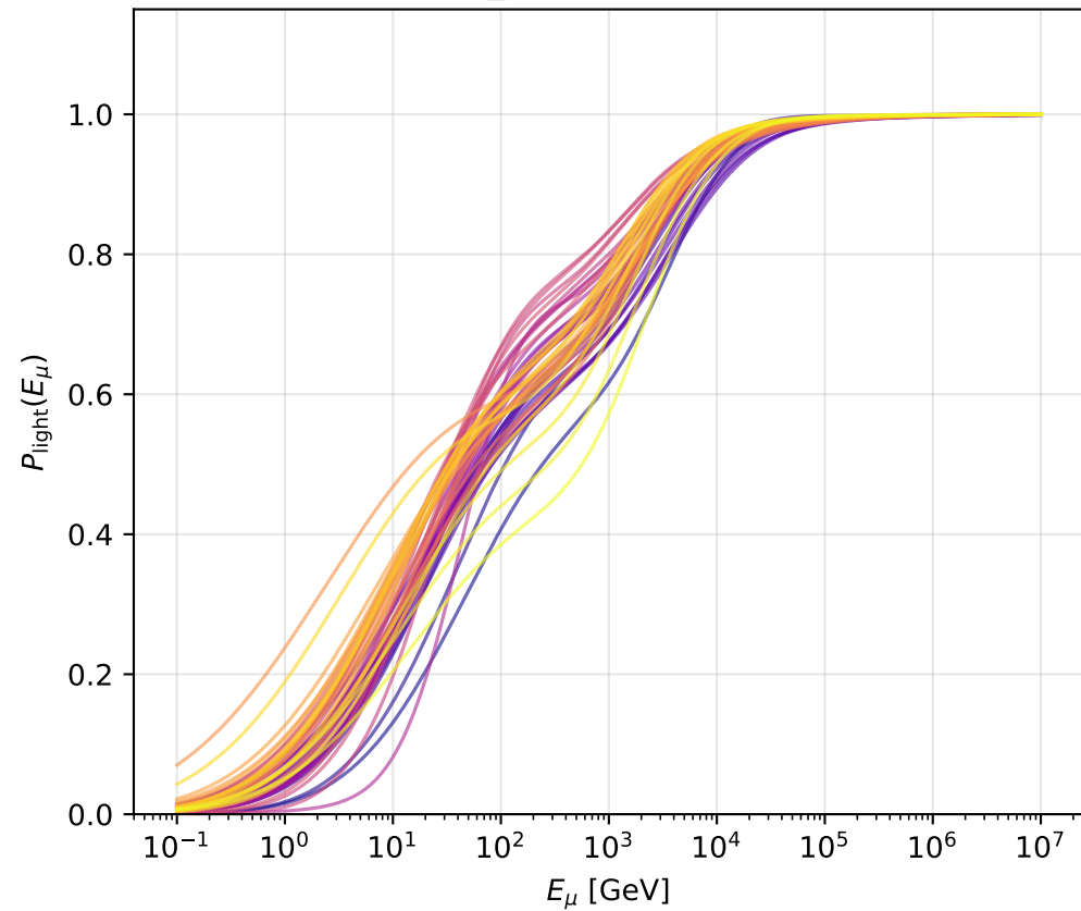
New — modified_sigmoid (50 slices, goes to 0)
