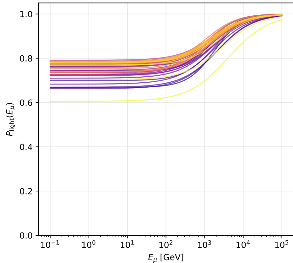
HESE depth-dependent P_{\text{light}} — sigmoid_Tianlu fits (39 depth slices)
