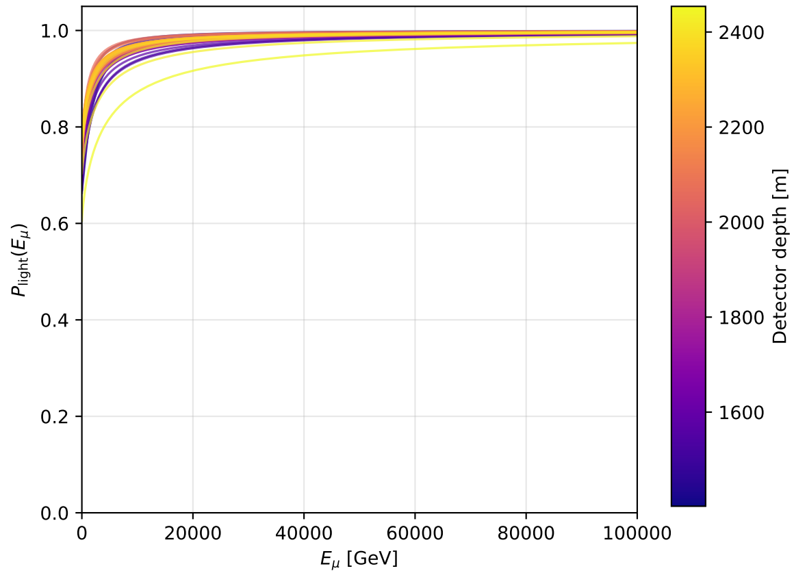
HESE depth-dependent P_{\text{light}} — sigmoid_Tianlu fits (39 depth slices)
