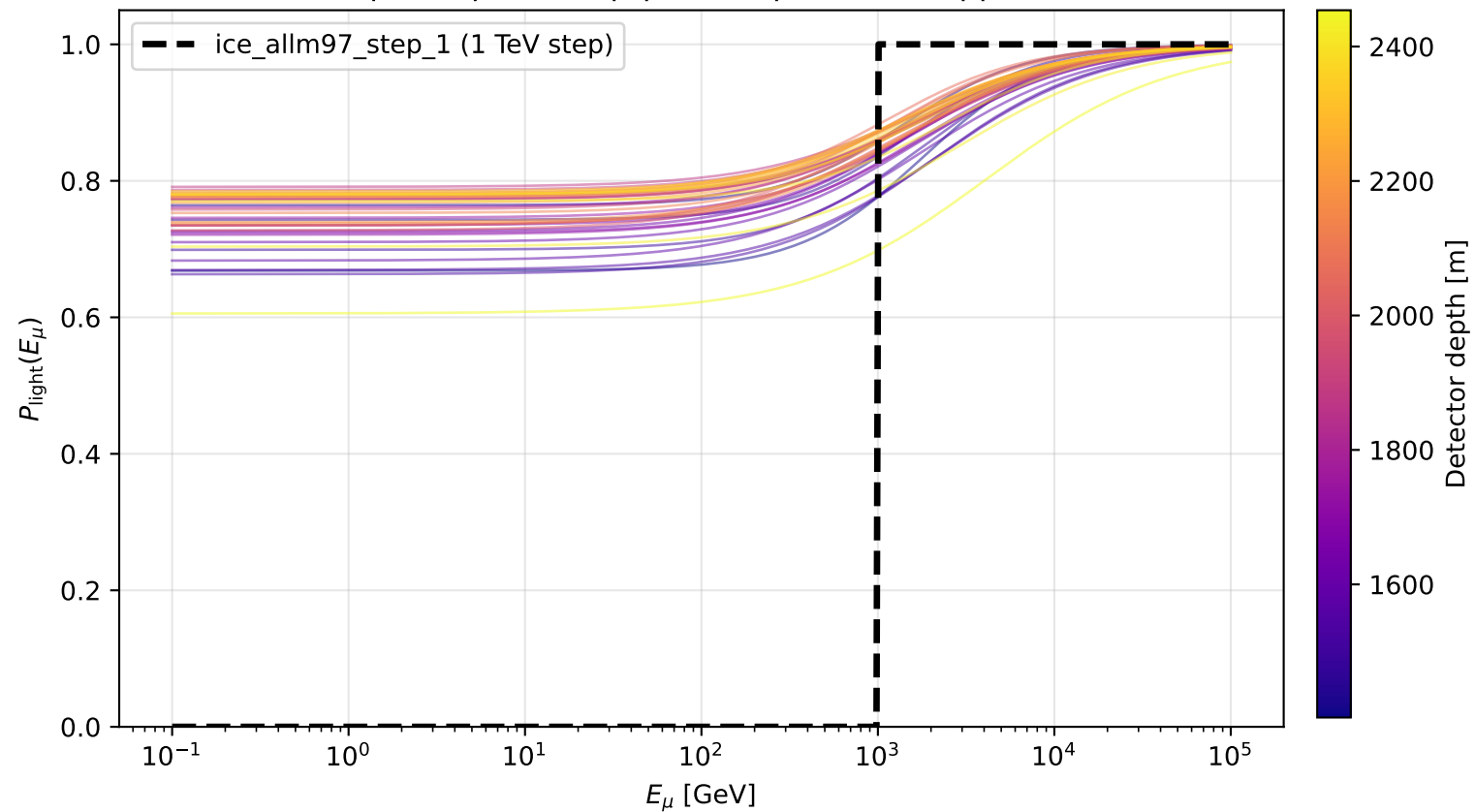
HESE depth-dependent prpl vs step-function approximation
