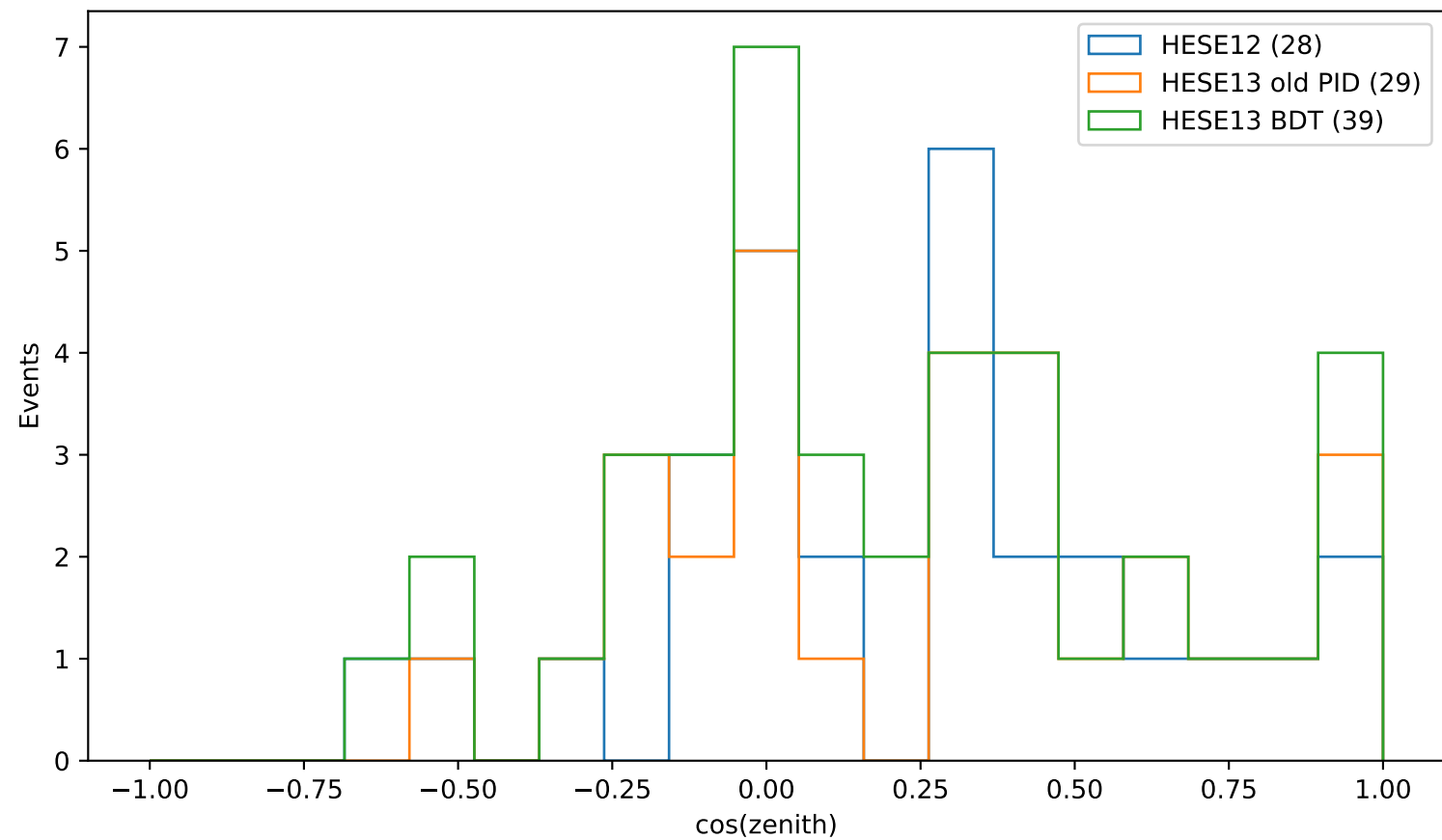
Track \cos(\text{zenith}) — all events
