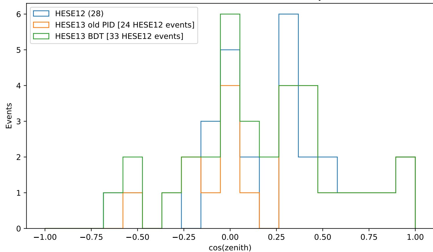
Track \cos(\text{zenith}) — HESE12 events only
