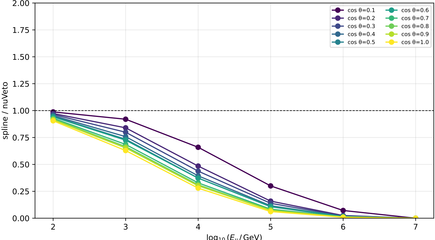
Ratio spline/nuVeto vs energy — conv nu e | depth=1950.0 m
