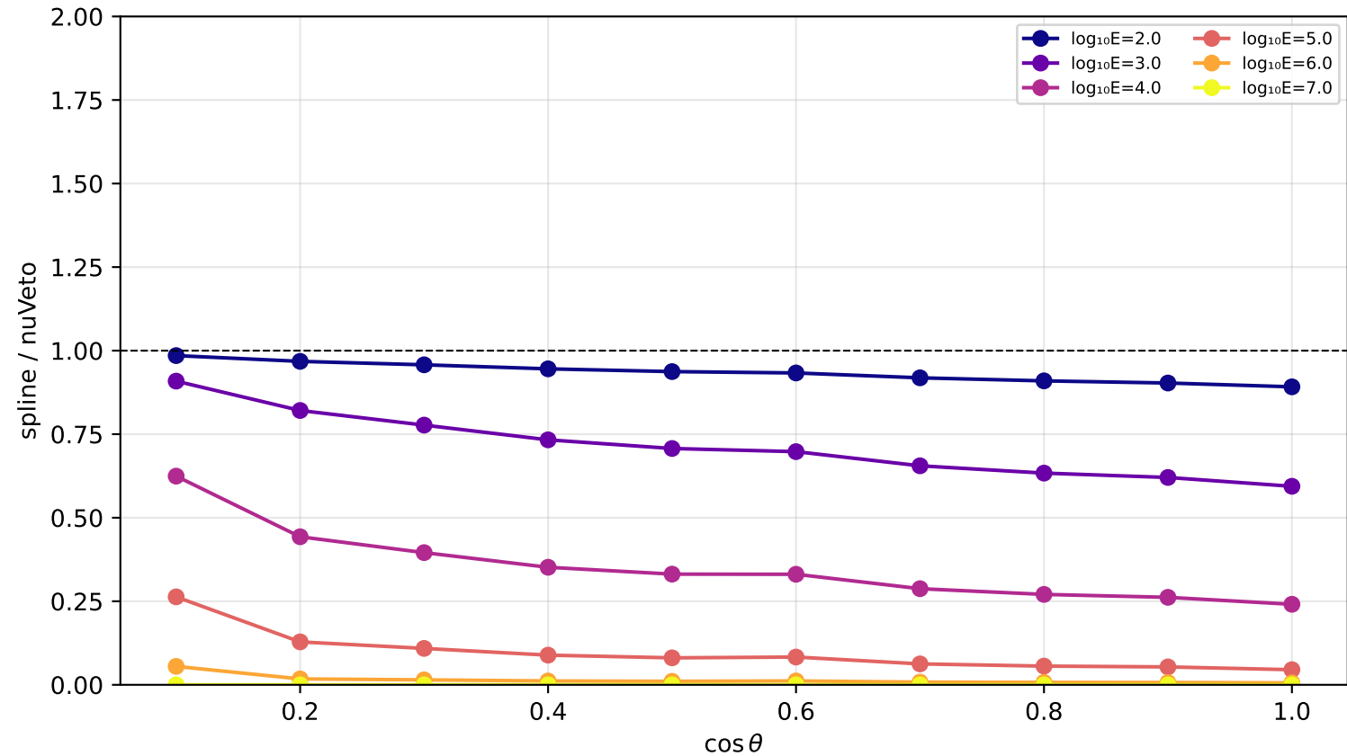
Ratio spline/nuVeto vs \cos \theta — conv nu_ebar | depth=1950.0 m
