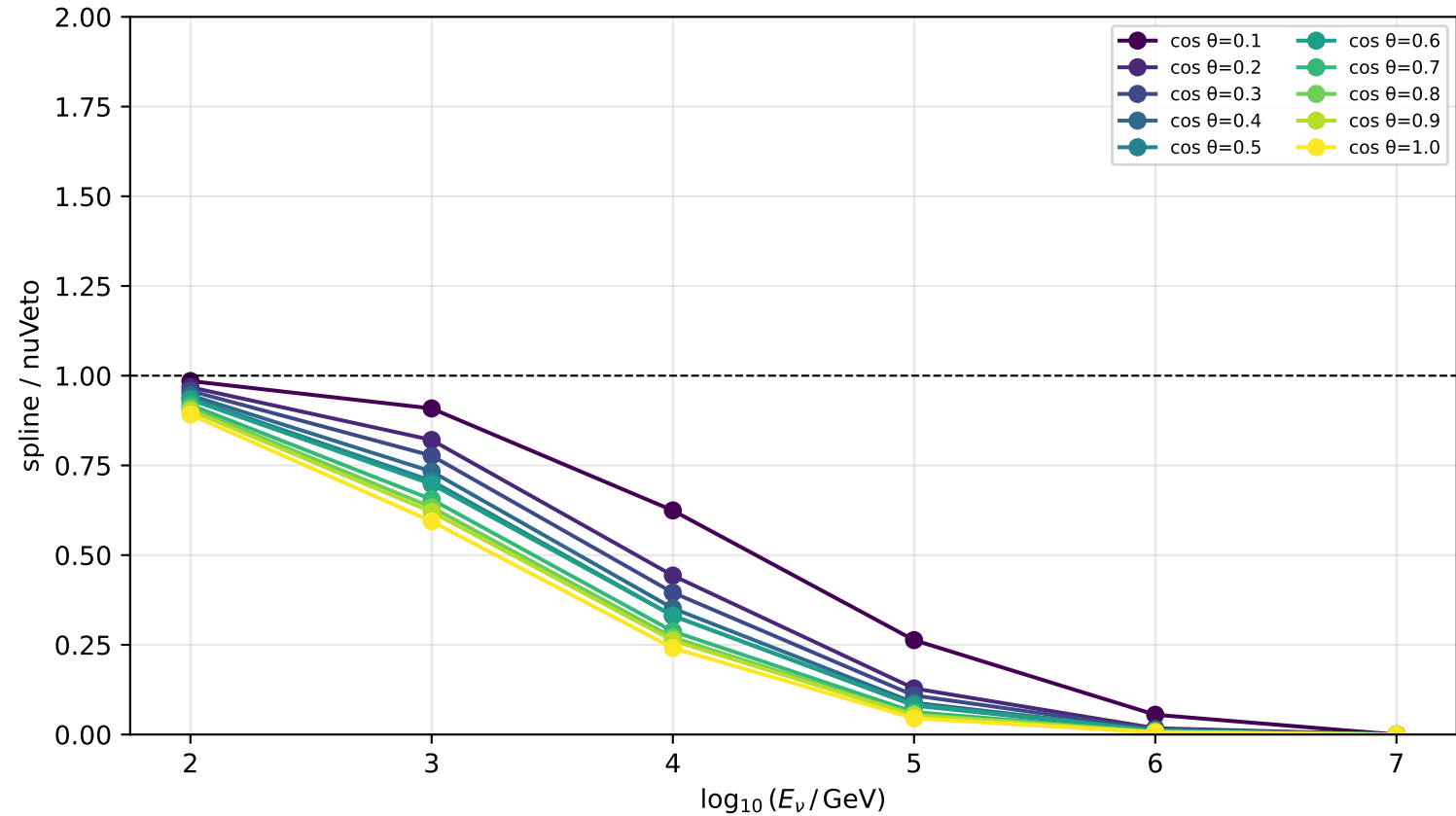
Ratio spline/nuVeto vs energy — conv nu_ebar | depth=1950.0 m
