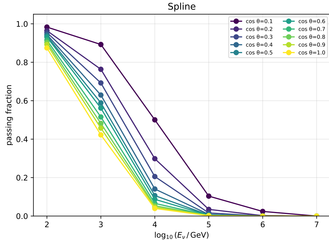
PF vs energy — conv nu mu | depth=1950.0 m
