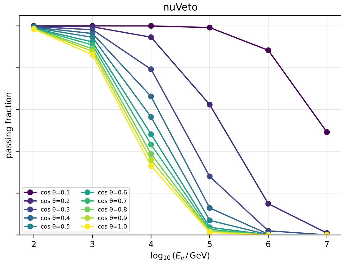
PF vs energy — conv nu mu | depth=1950.0 m
