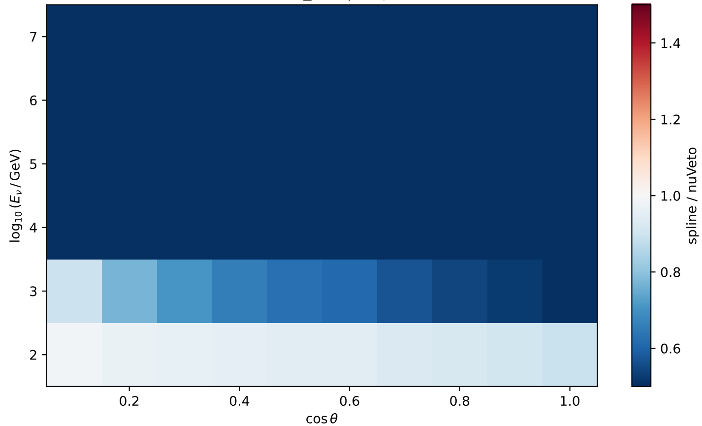
Ratio 2D — conv nu_mu | depth=1950.0 m
