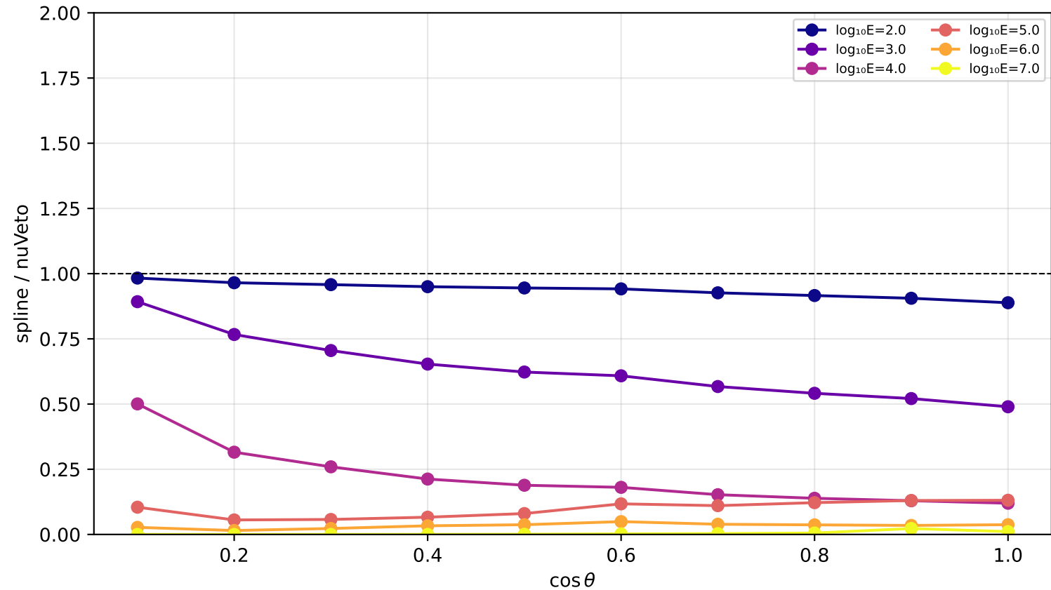
Ratio spline/nuVeto vs \cos \theta — conv nu_mu | depth=1950.0 m
