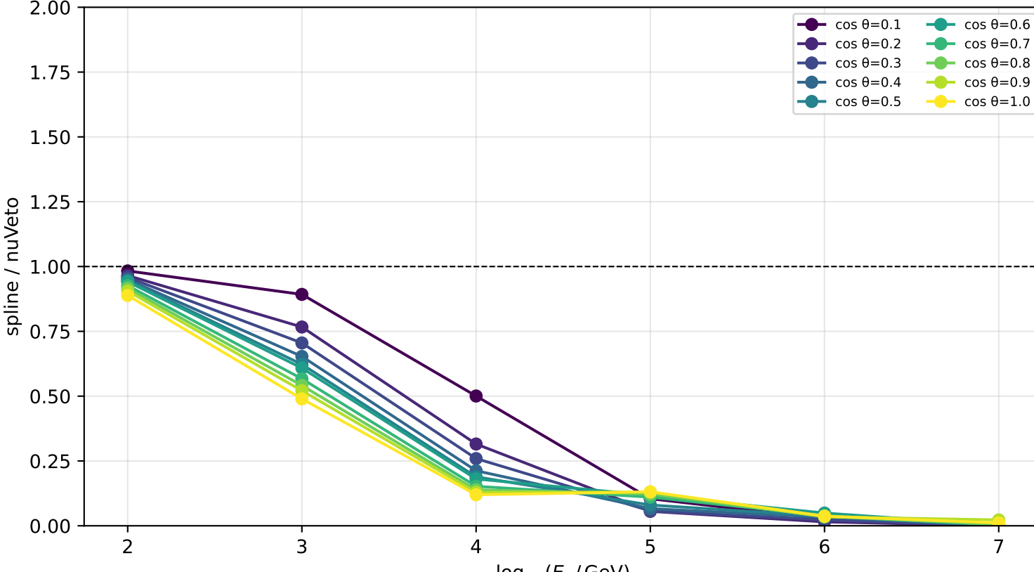
Ratio spline/nuVeto vs energy — conv nu mu | depth=1950.0 m
