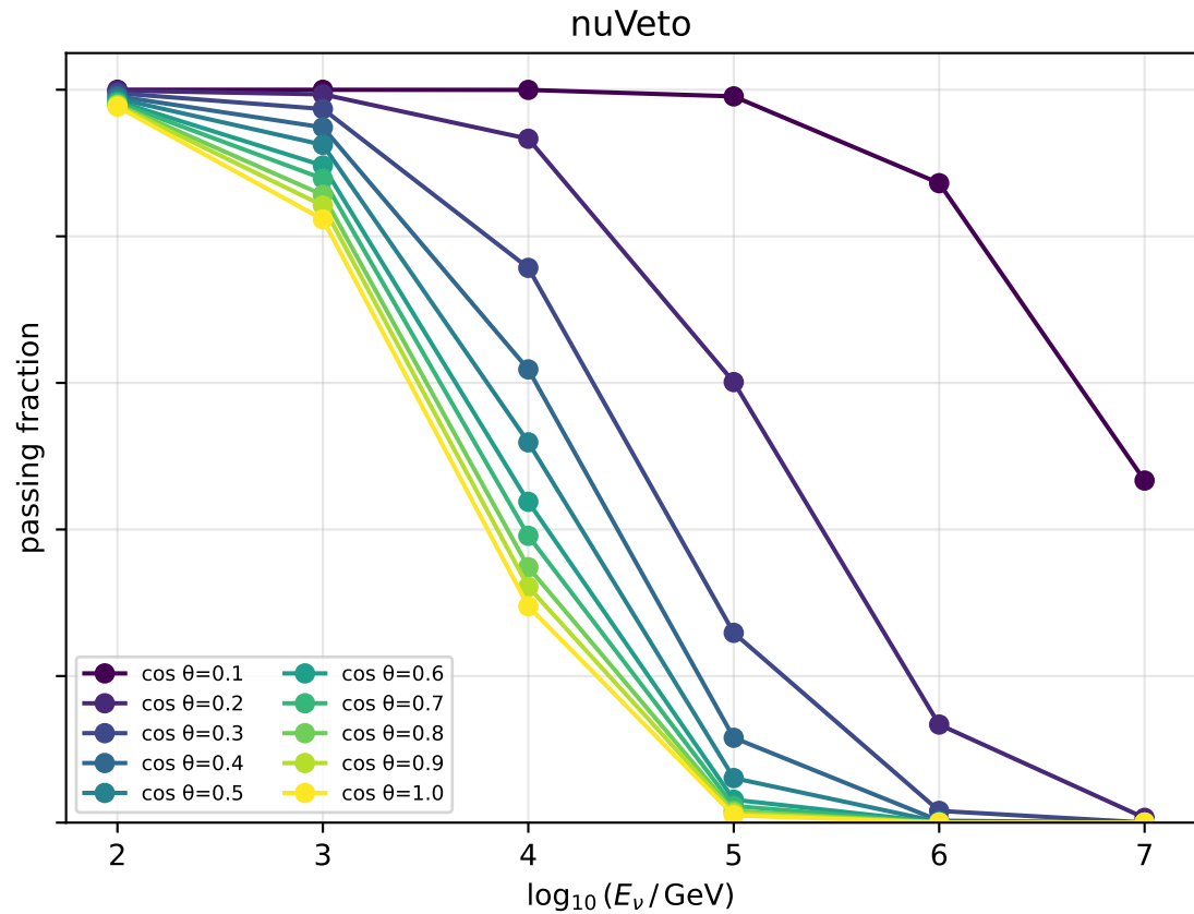
PF vs energy — conv nu_mubar | depth=1950.0 m
