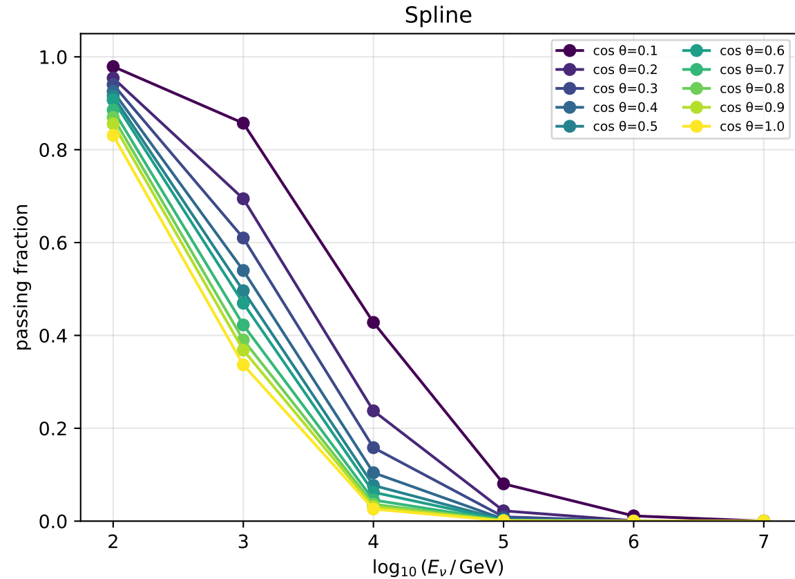
PF vs energy — conv nu_mubar | depth=1950.0 m
