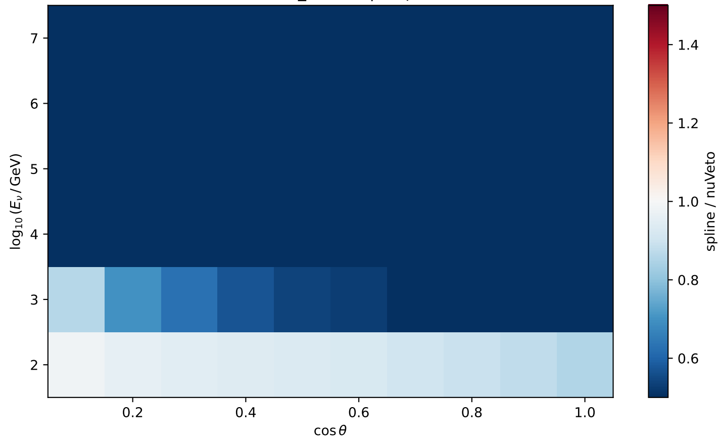
Ratio 2D — conv nu_mubar | depth=1950.0 m
