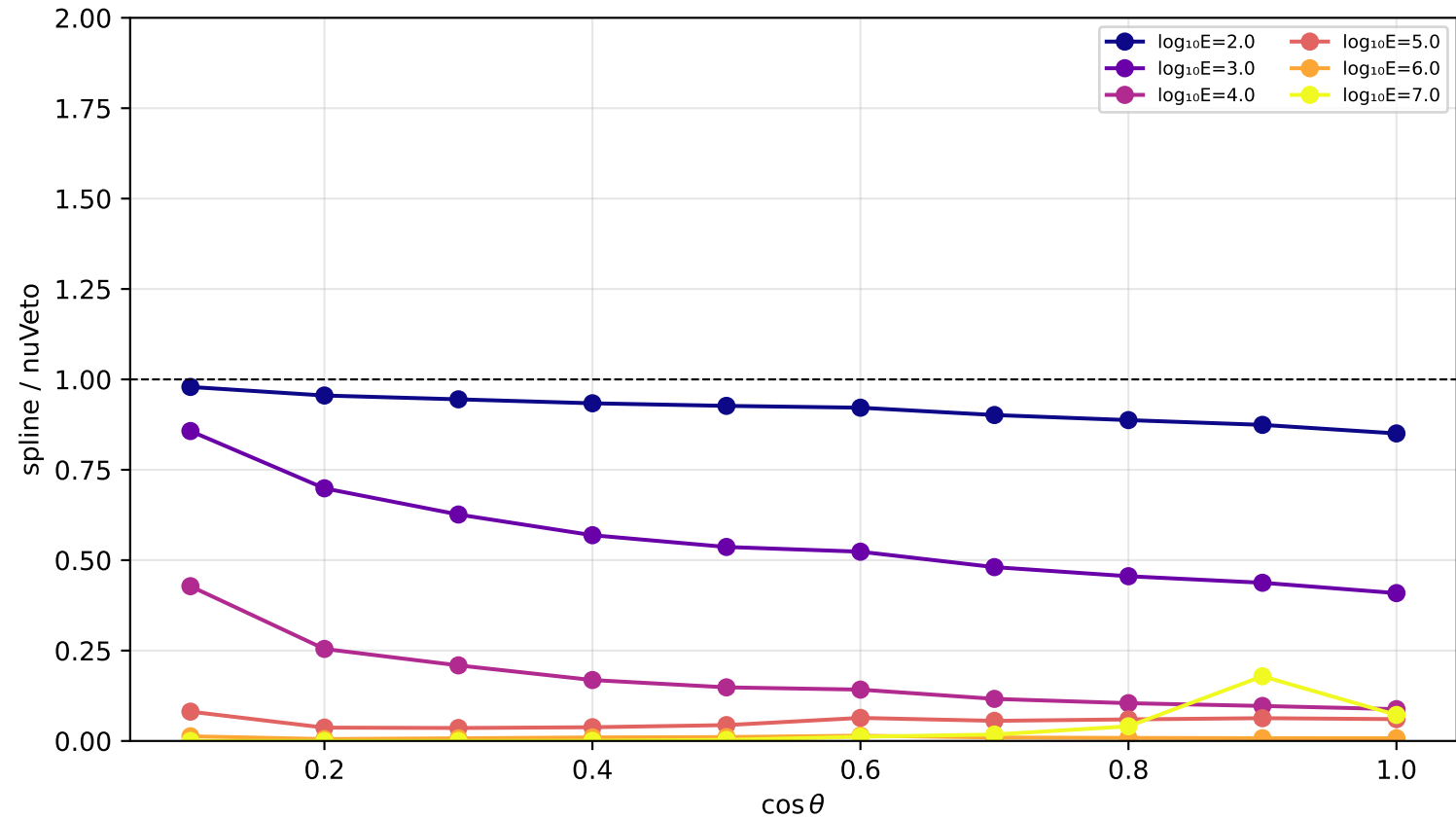
Ratio spline/nuVeto vs \cos \theta — conv nu_mubar | depth=1950.0 m
