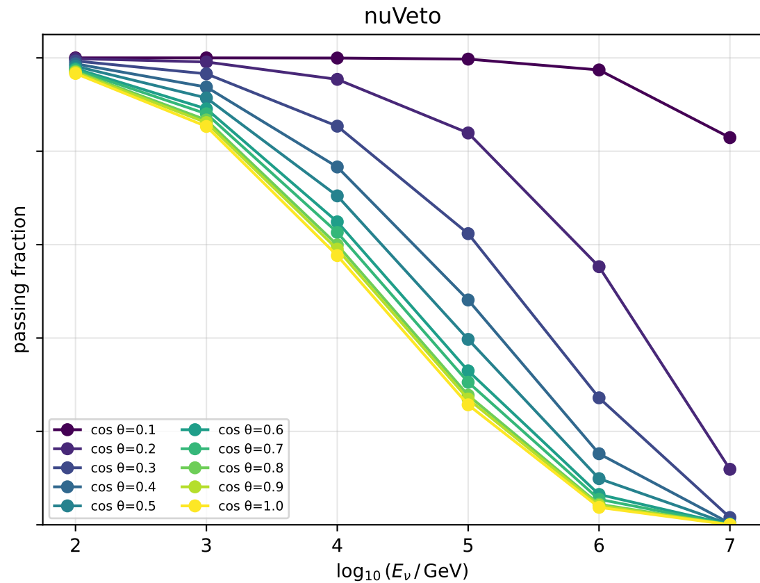
PF vs energy — pr nu_e | depth=1950.0 m
