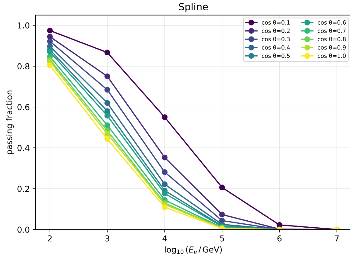
PF vs energy — pr nu_e | depth=1950.0 m
