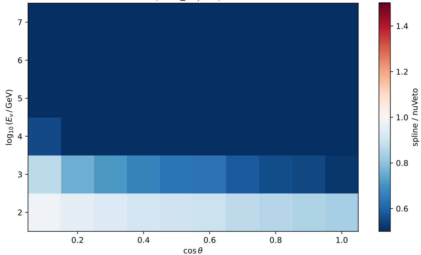
Ratio 2D — pr nu_e | depth=1950.0 m
