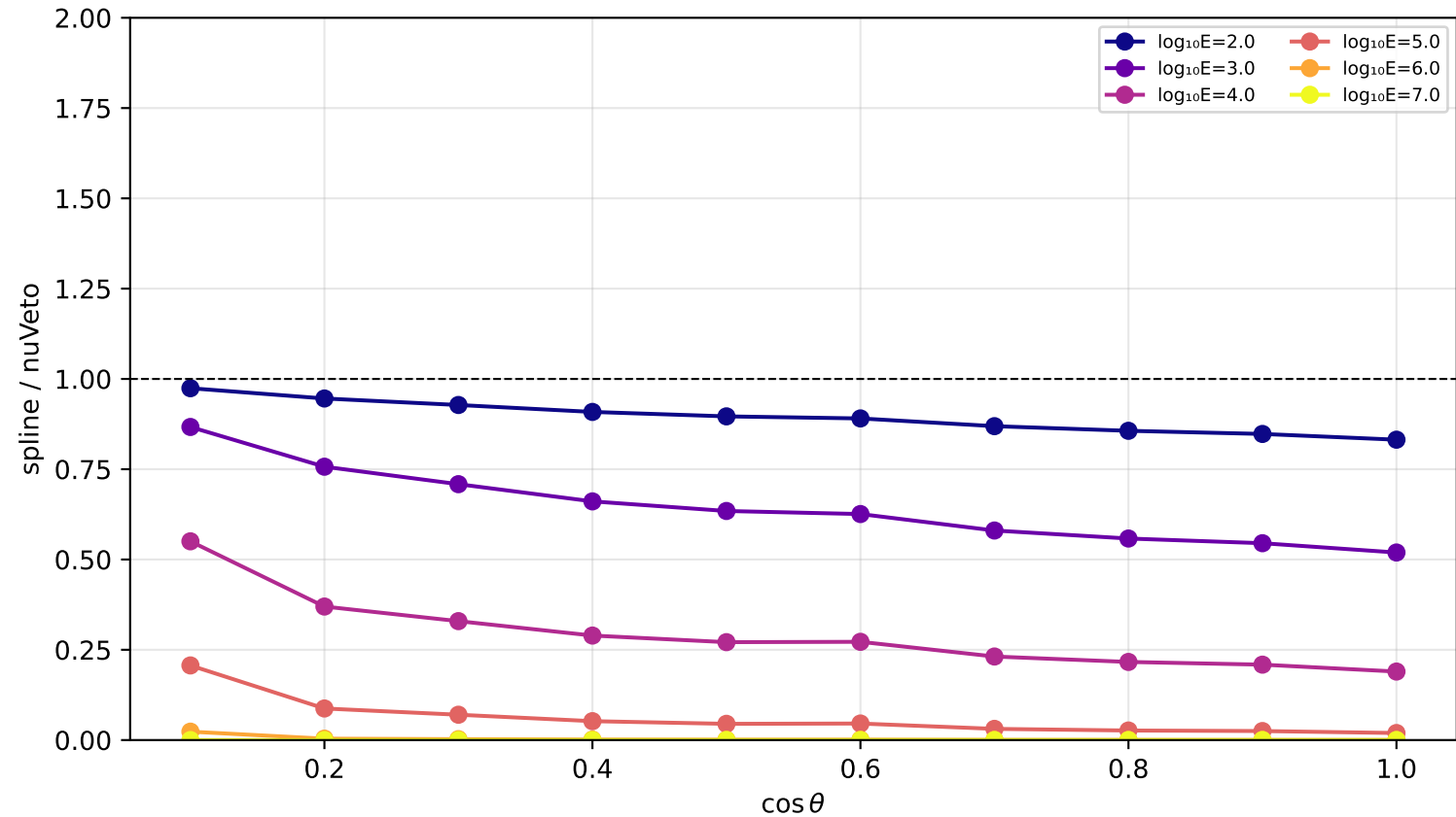
Ratio spline/nuVeto vs \cos \theta — pr nu_e | depth=1950.0 m
