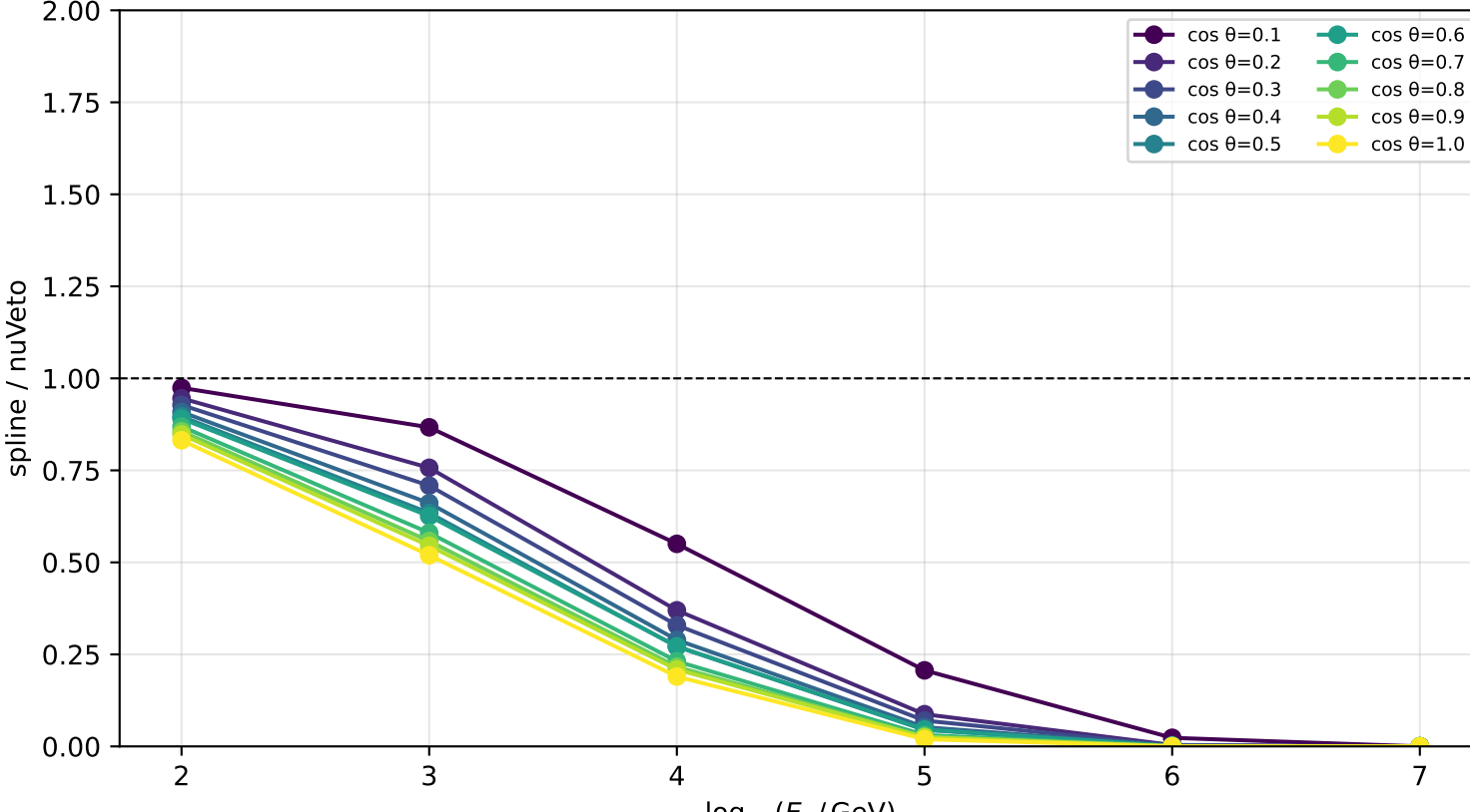
Ratio spline/nuVeto vs energy — pr nu_e | depth=1950.0 m
