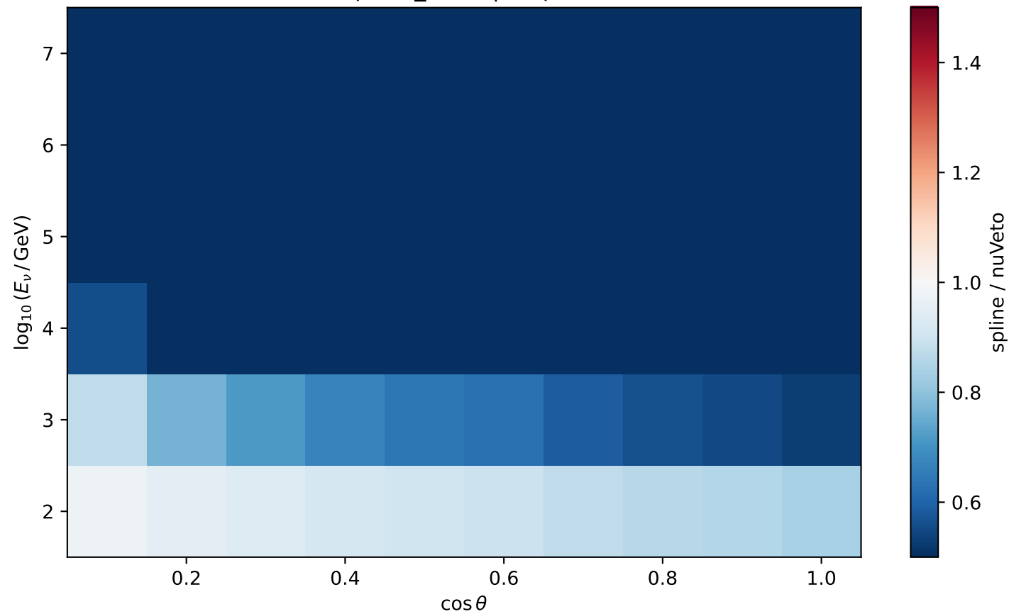
Ratio 2D — pr nu_ebar | depth=1950.0 m
