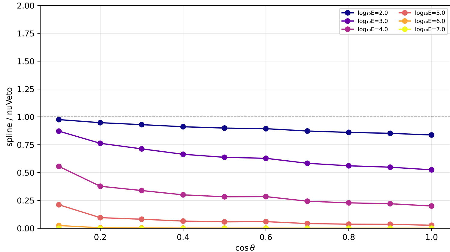
Ratio spline/nuVeto vs \cos \theta — pr nu_ubar | depth=1950.0 m
