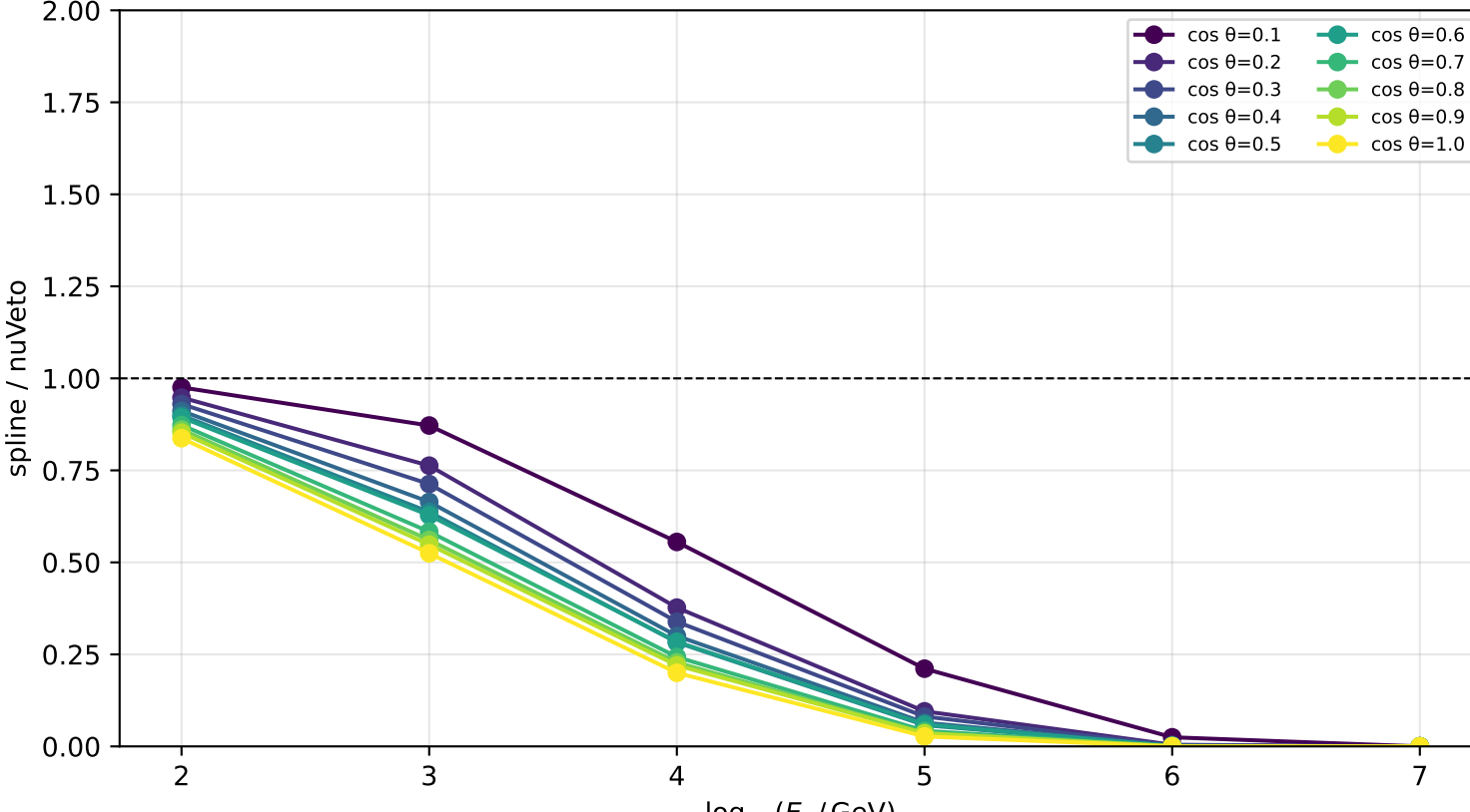
Ratio spline/nuVeto vs energy — pr nu ebar | depth=1950.0 m
