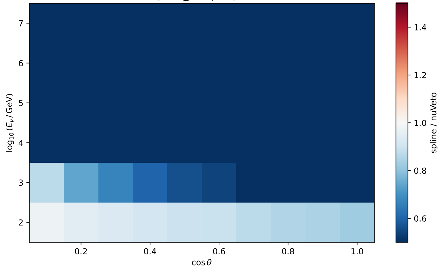
Ratio 2D — pr nu_mu | depth=1950.0 m
