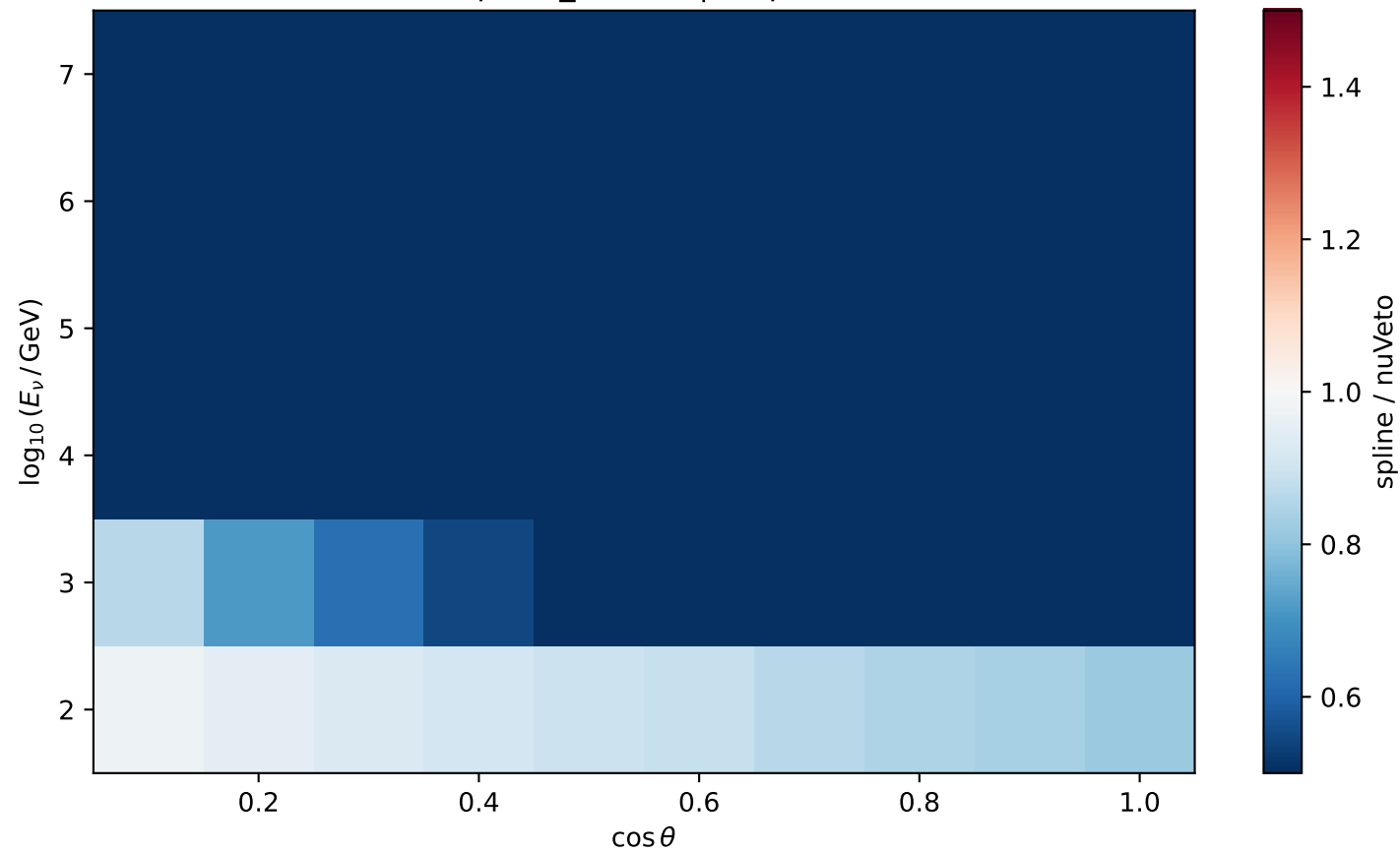
Ratio 2D — pr nu_mubar | depth=1950.0 m
