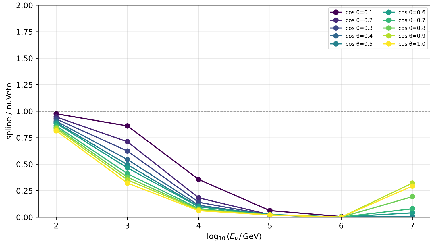
Ratio spline/nuVeto vs energy — pr nu_mubar | depth=1950.0 m
