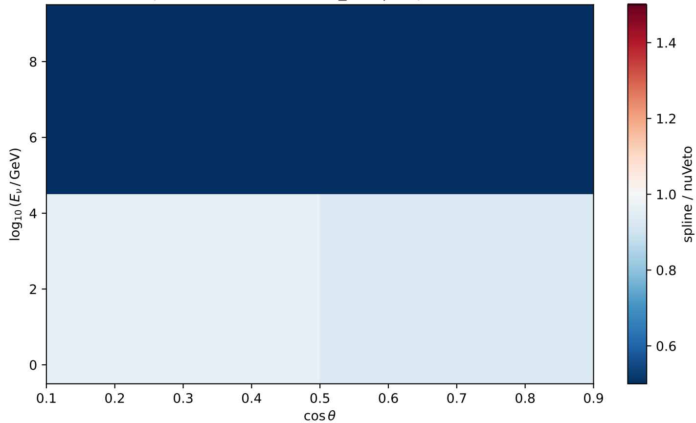
Ratio spline/nuVeto — conv nu_mu | depth = 1950.0 m
