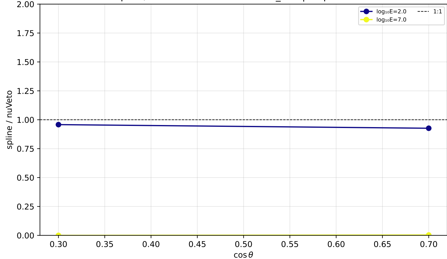
Ratio spline/nuVeto vs \cos \theta — conv nu_mu | depth = 1950.0 m
