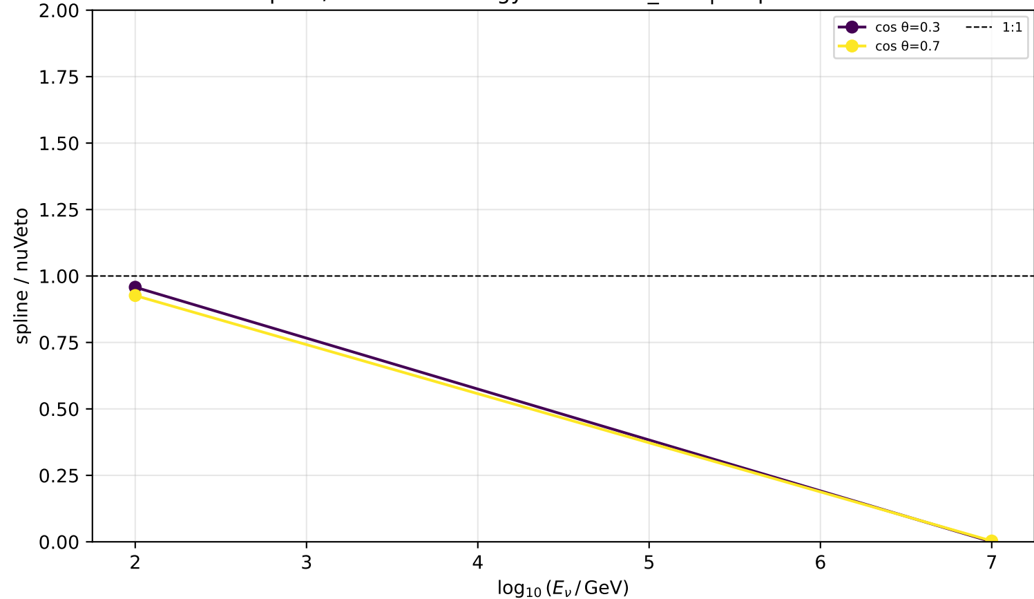
Ratio spline/nuVeto vs energy — conv nu_mu | depth = 1950.0 m
