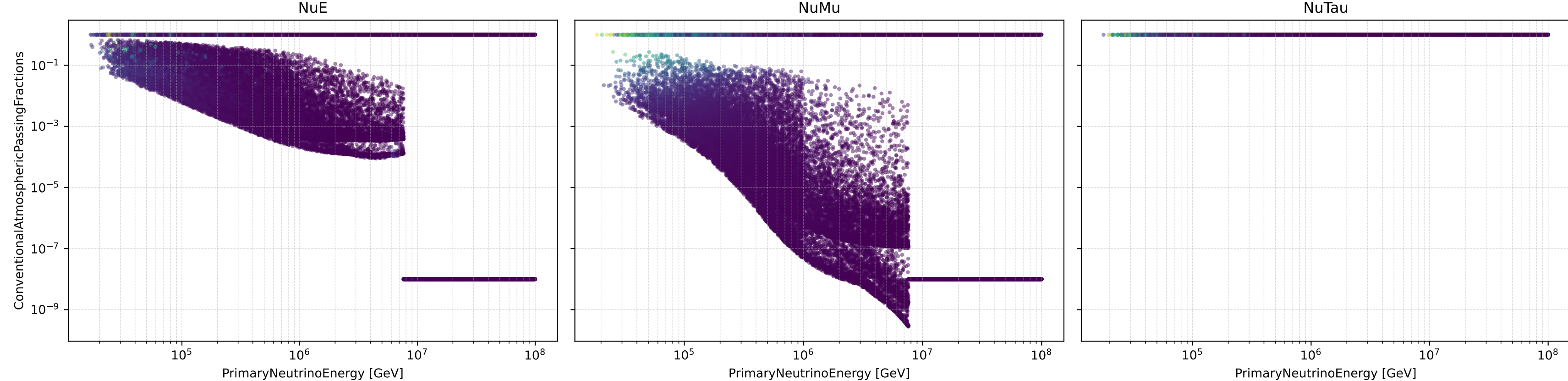
PrimaryNeutrinoEnergy [GeV] vs ConventionalAtmosphericPassingFractions (Spice)
