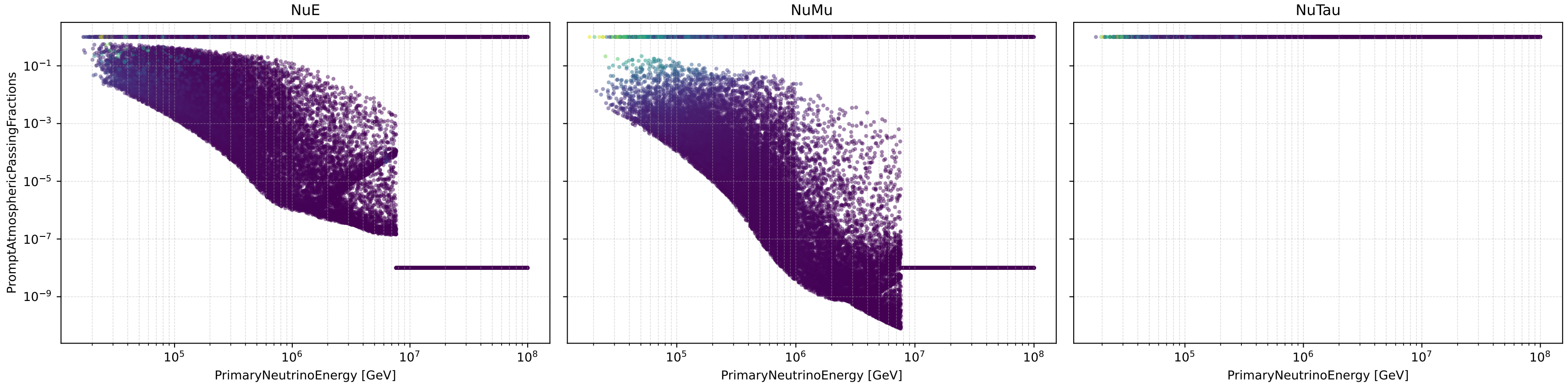
PrimaryNeutrinoEnergy [GeV] vs PromptAtmosphericPassingFractions (Spice)
