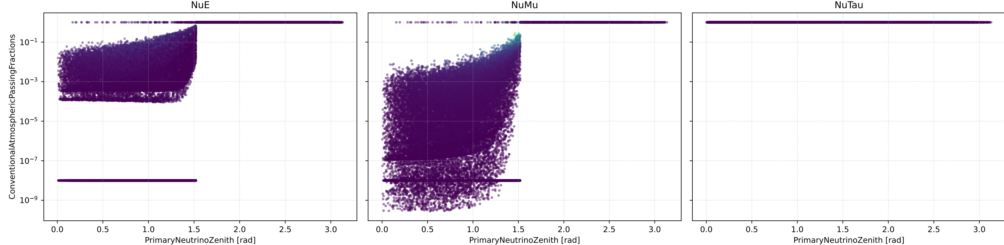
PrimaryNeutrinoZenith [rad] vs ConventionalAtmosphericPassingFractions (Spice)
