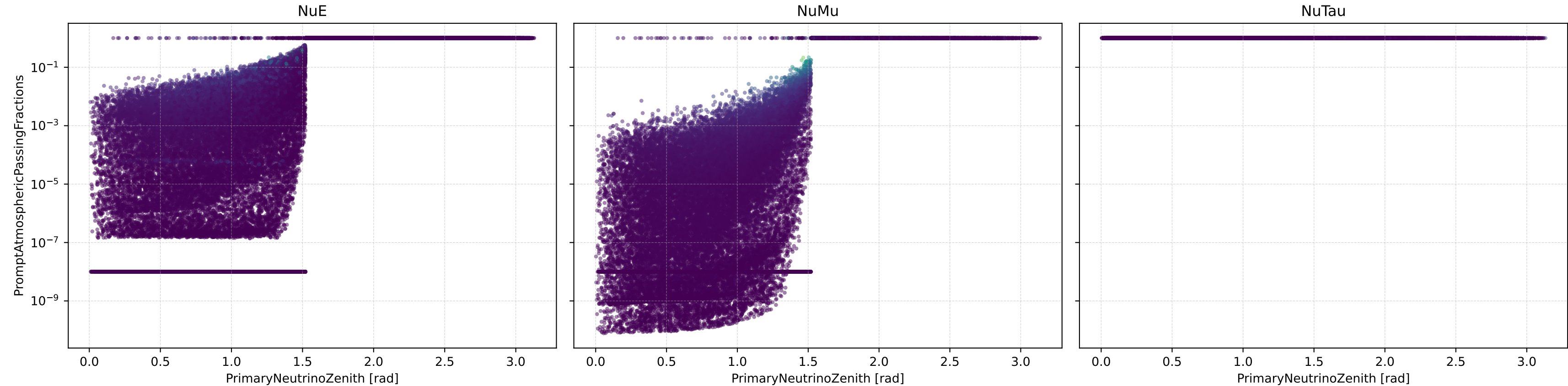
PrimaryNeutrinoZenith [rad] vs PromptAtmosphericPassingFractions (Spice)
